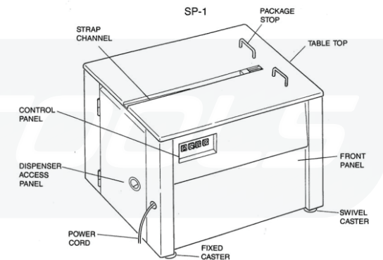
FIGURE 1. MAJOR COMPONENTS, EXTERIOR
