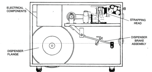
FIGURE 2. MAJOR COMPONENTS, FRONT VIEW
